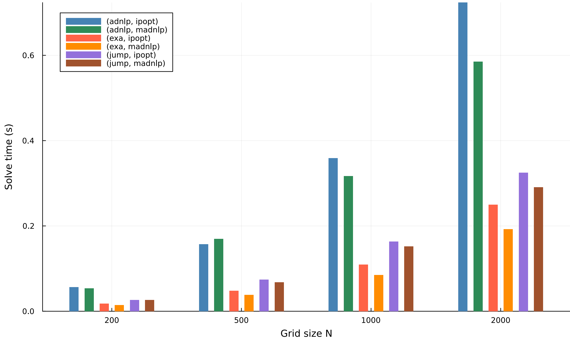
Solve time vs grid size (bar) — rocket
