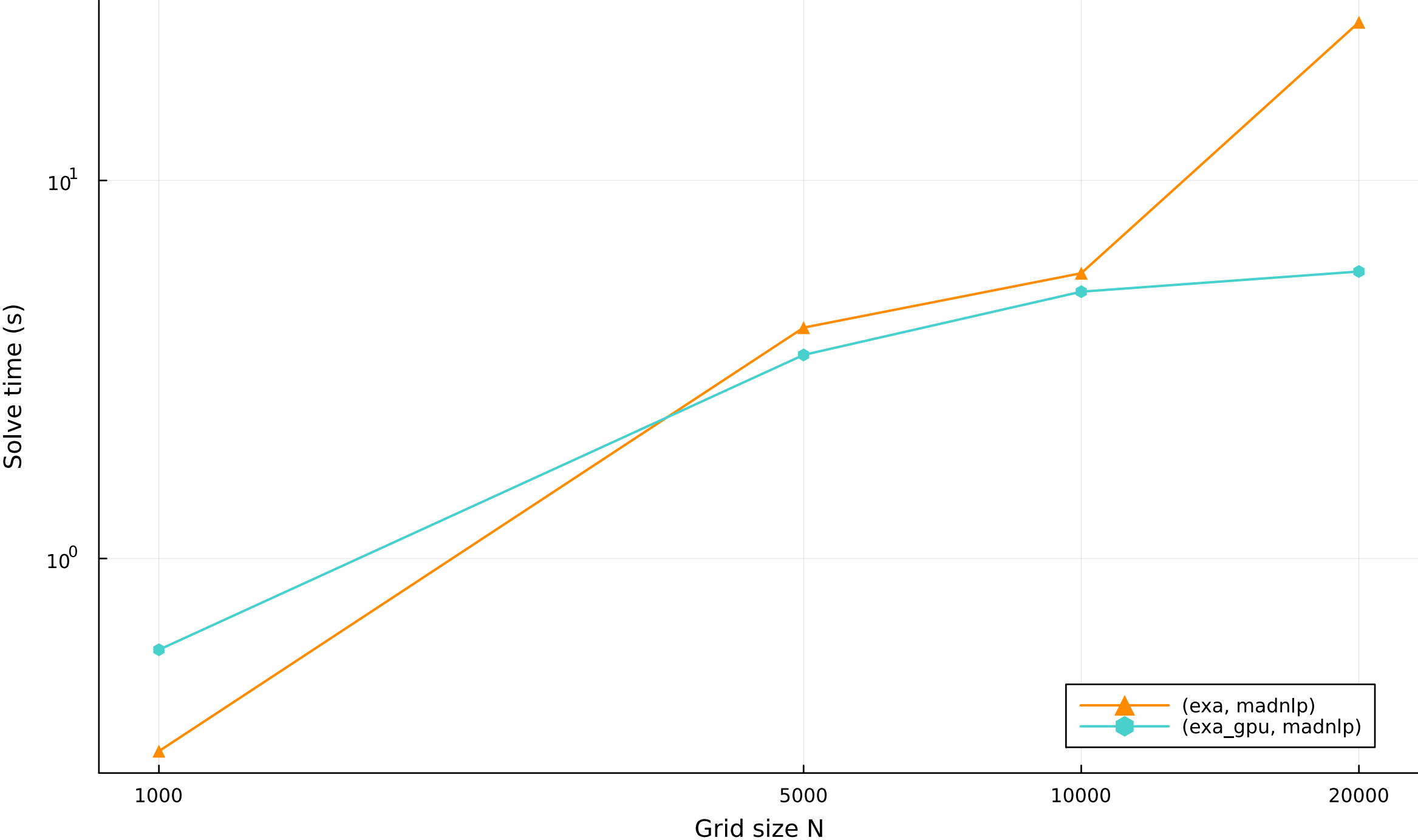
Solve time vs grid size — robot
