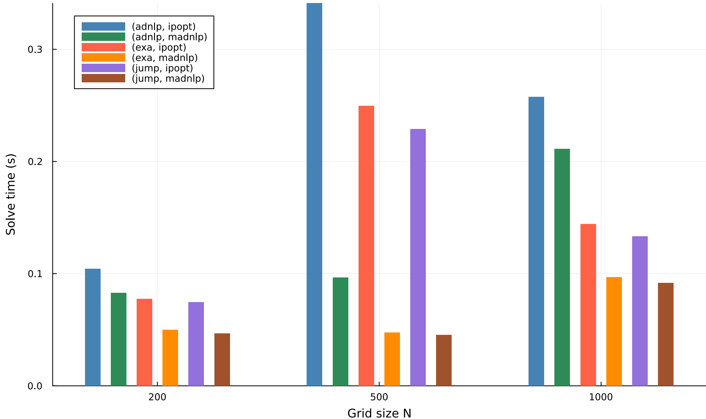
Solve time vs grid size (bar) — jackson
