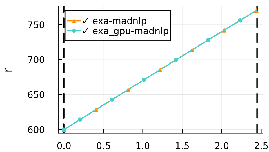
state
