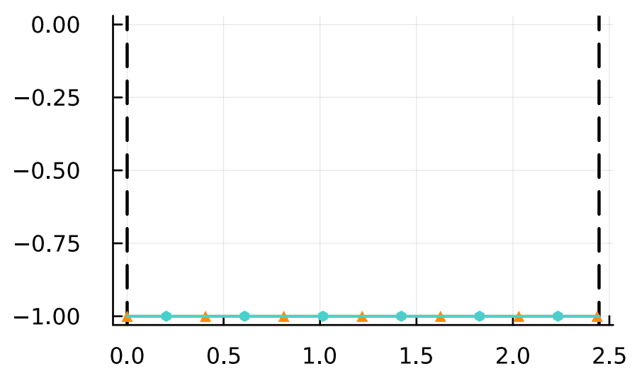
costate
