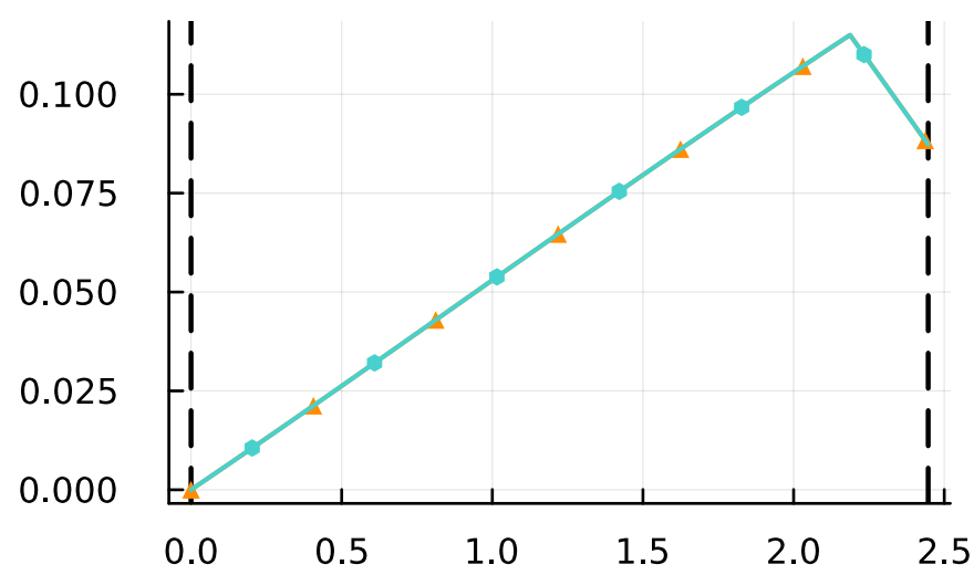
\gamma
