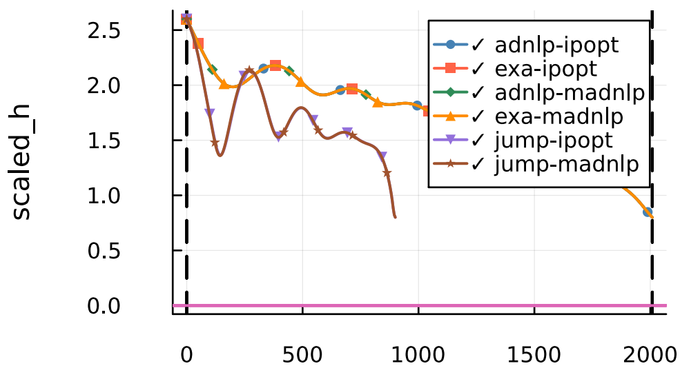
state
