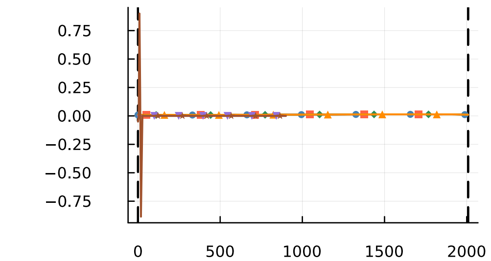
costate
