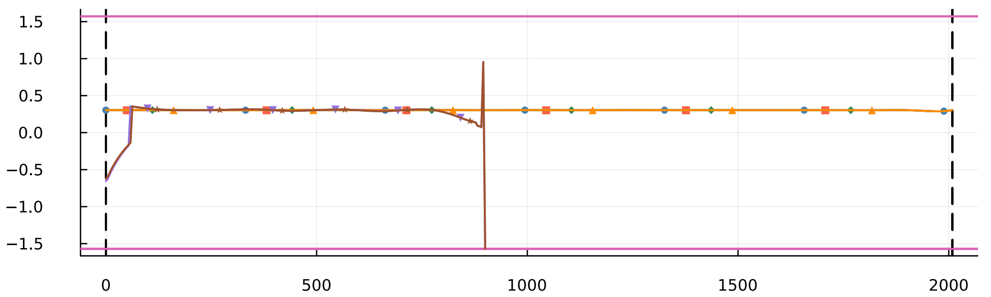
control
