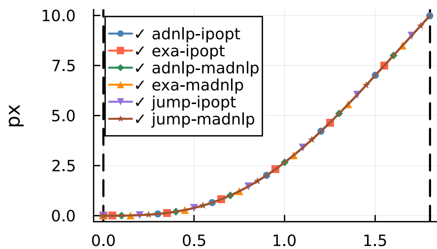
state
