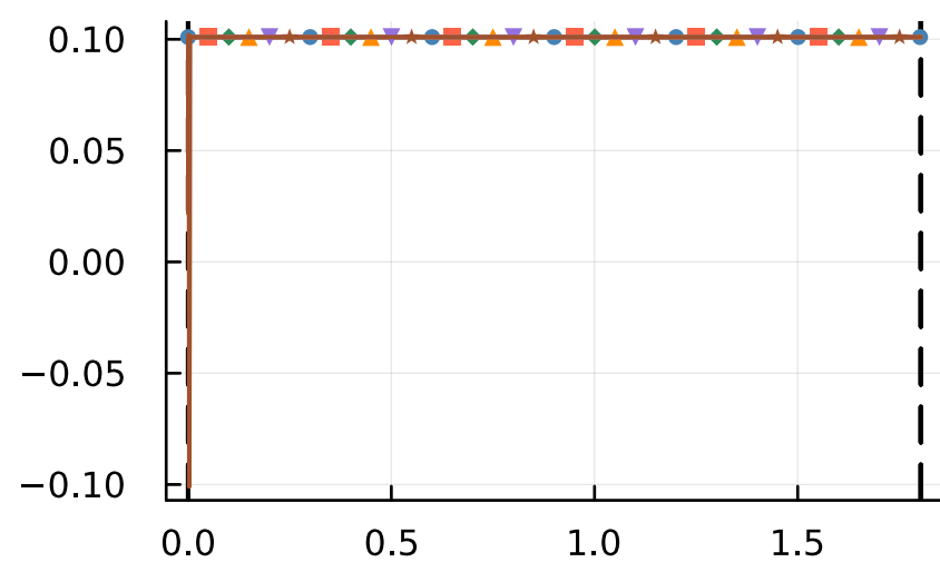
costate
