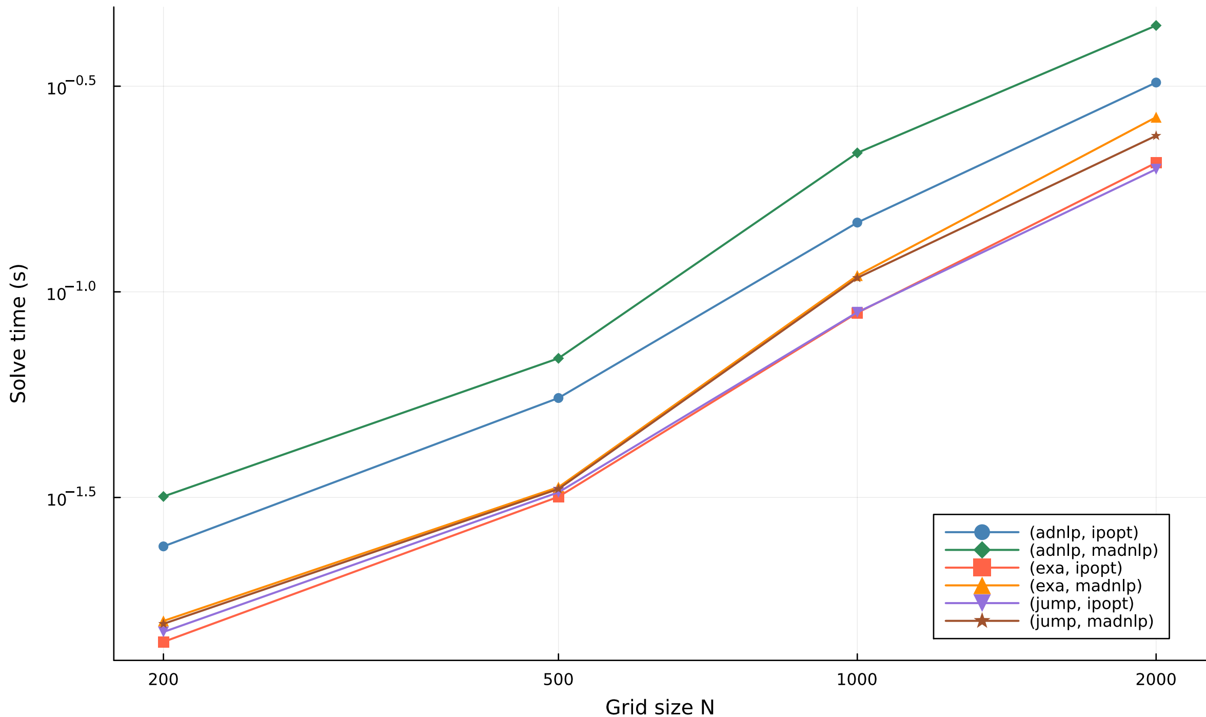
Solve time vs grid size — robbins
