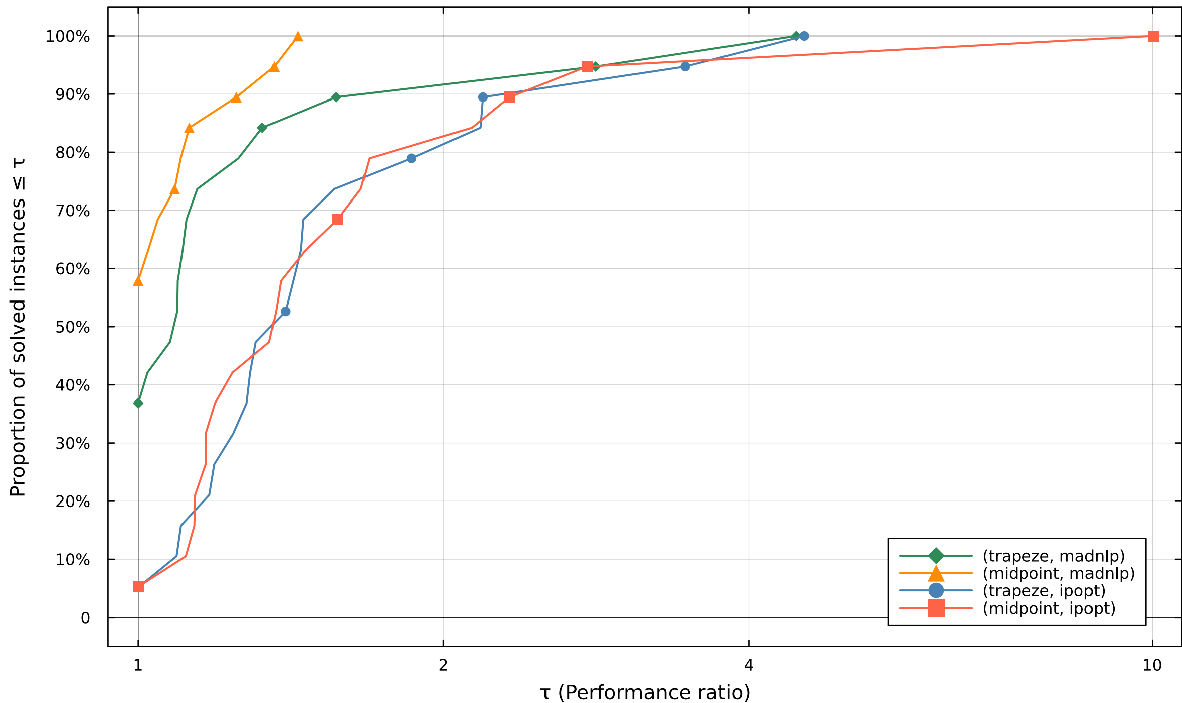
Performance profile — CPU time
