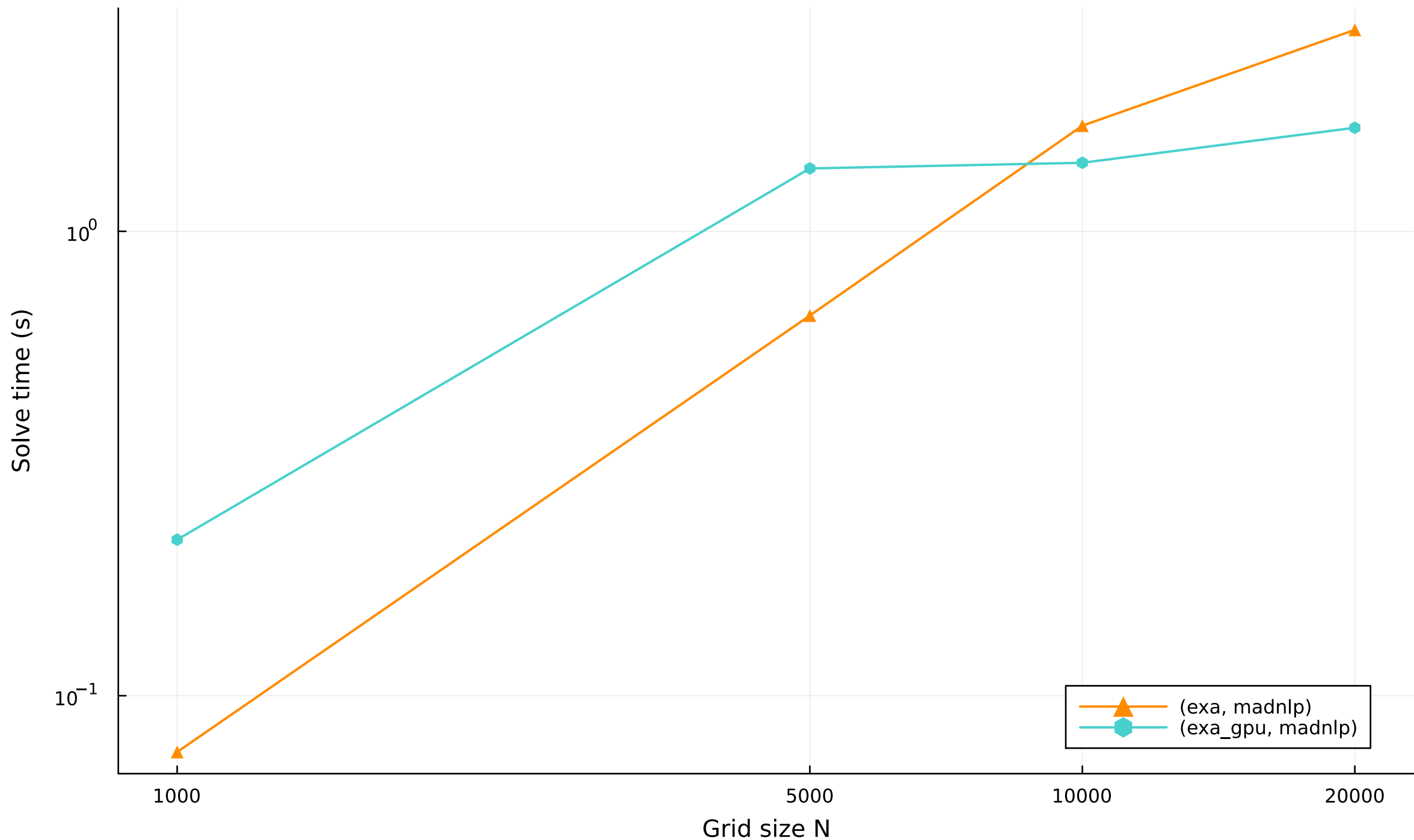
Solve time vs grid size — brachistochrone
