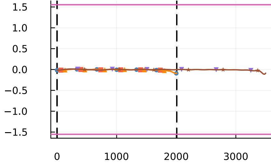
\gamma
