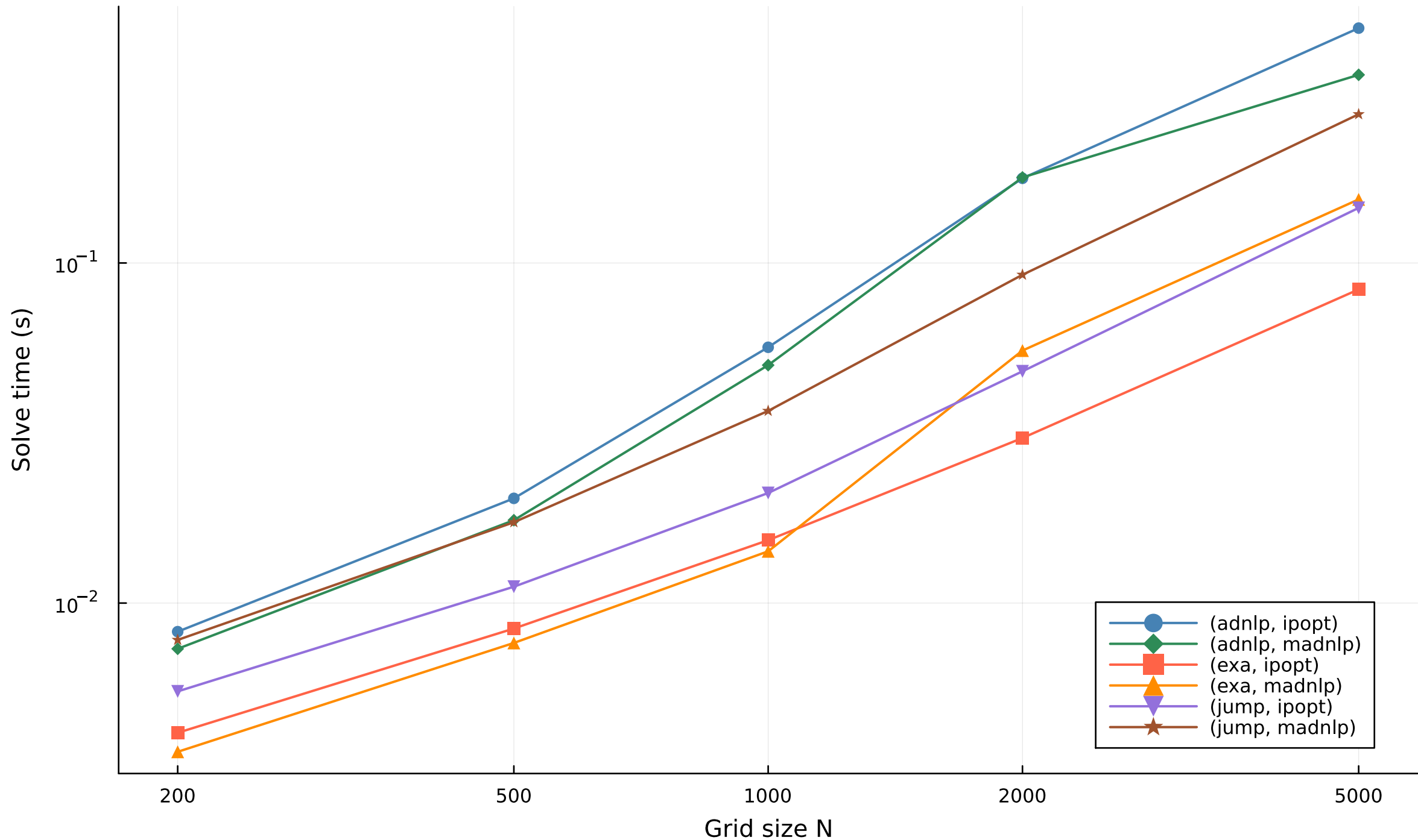
Solve time vs grid size — vanderpol
