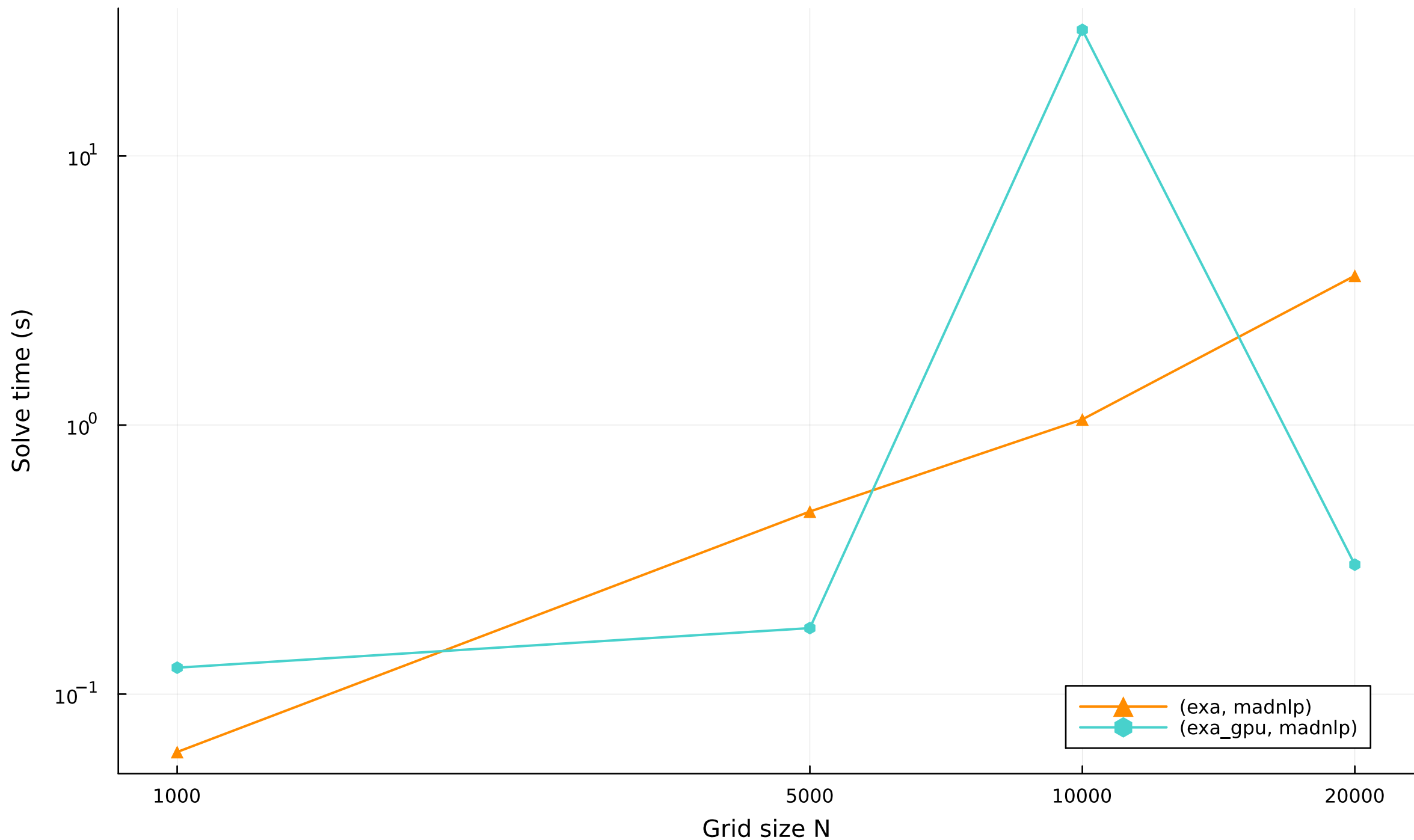
Solve time vs grid size — chain
