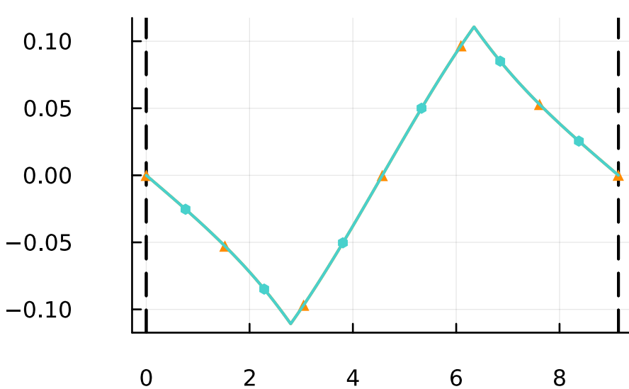
d\phi
