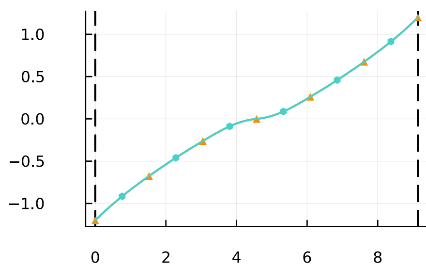
costate
