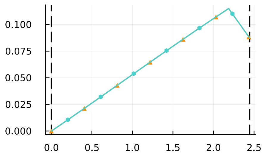
\gamma
