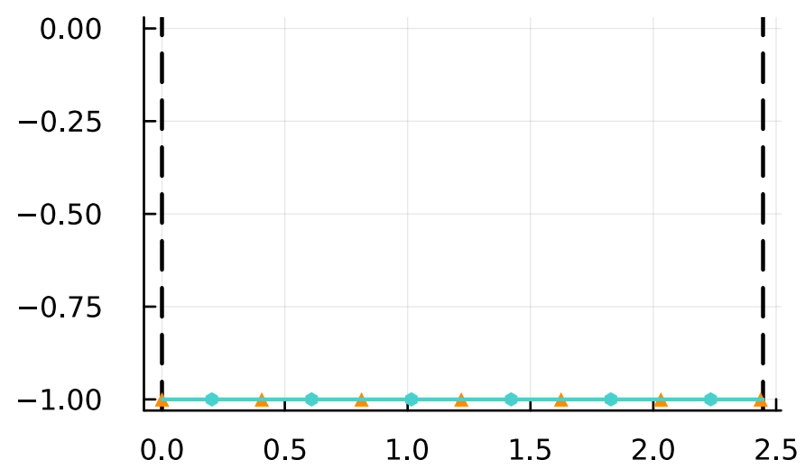
costate
