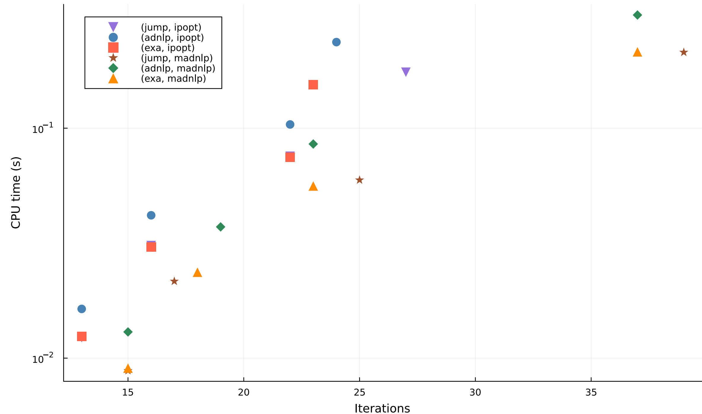
Iterations vs CPU time — bryson_denham
