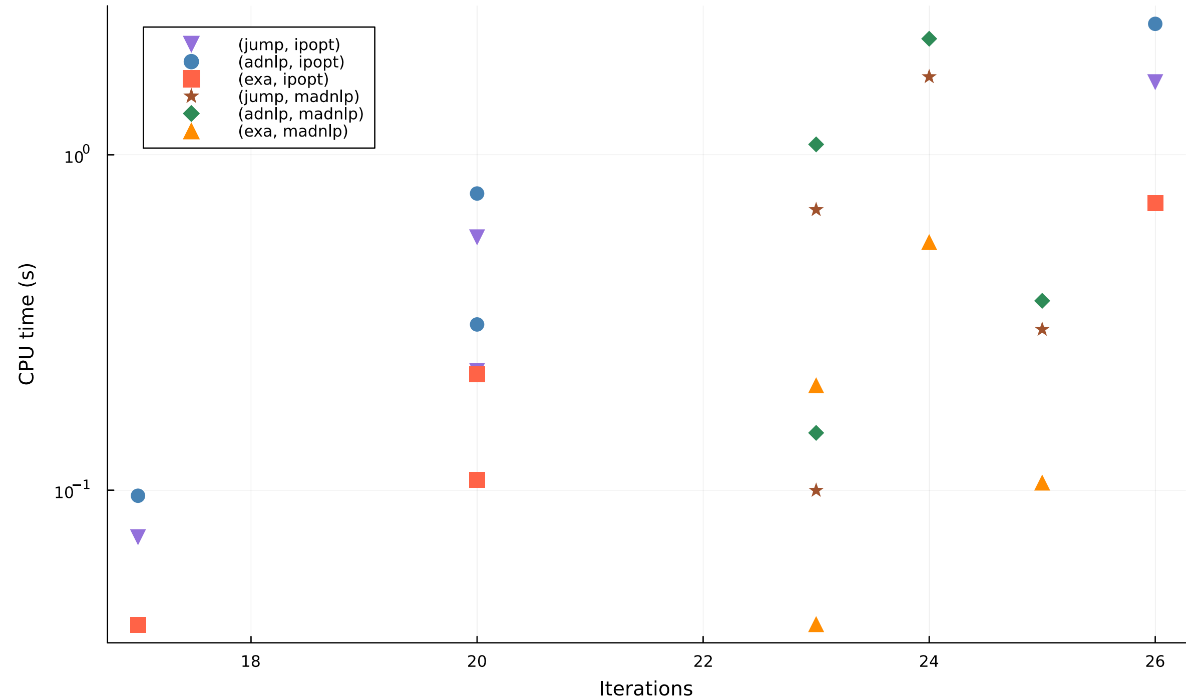
Iterations vs CPU time — balanced_field
