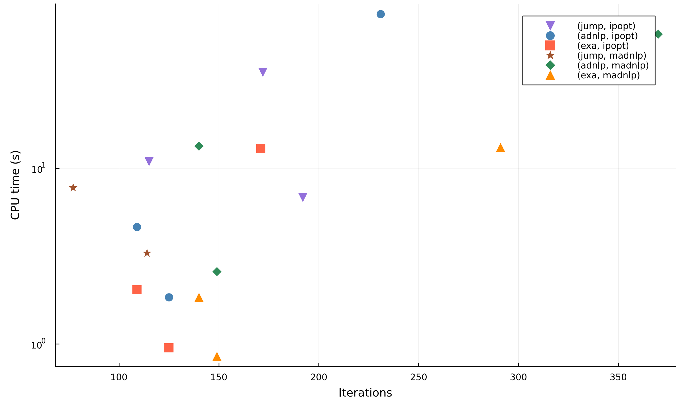
Iterations vs CPU time — space_shuttle
