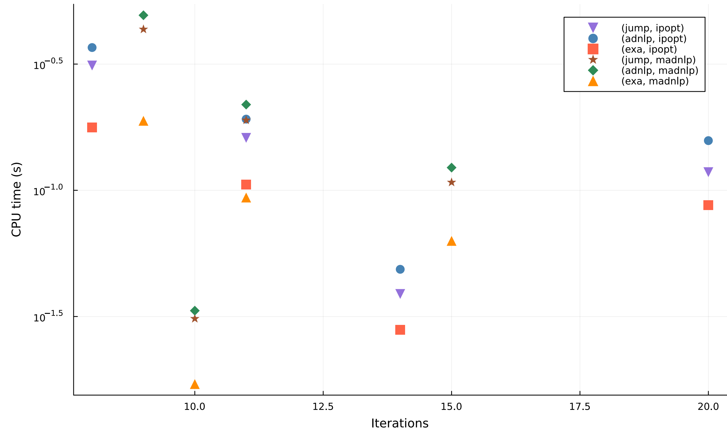
Iterations vs CPU time — brachistochrone
