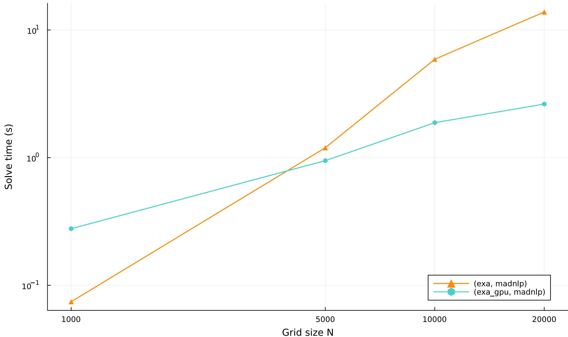
Solve time vs grid size — beam
