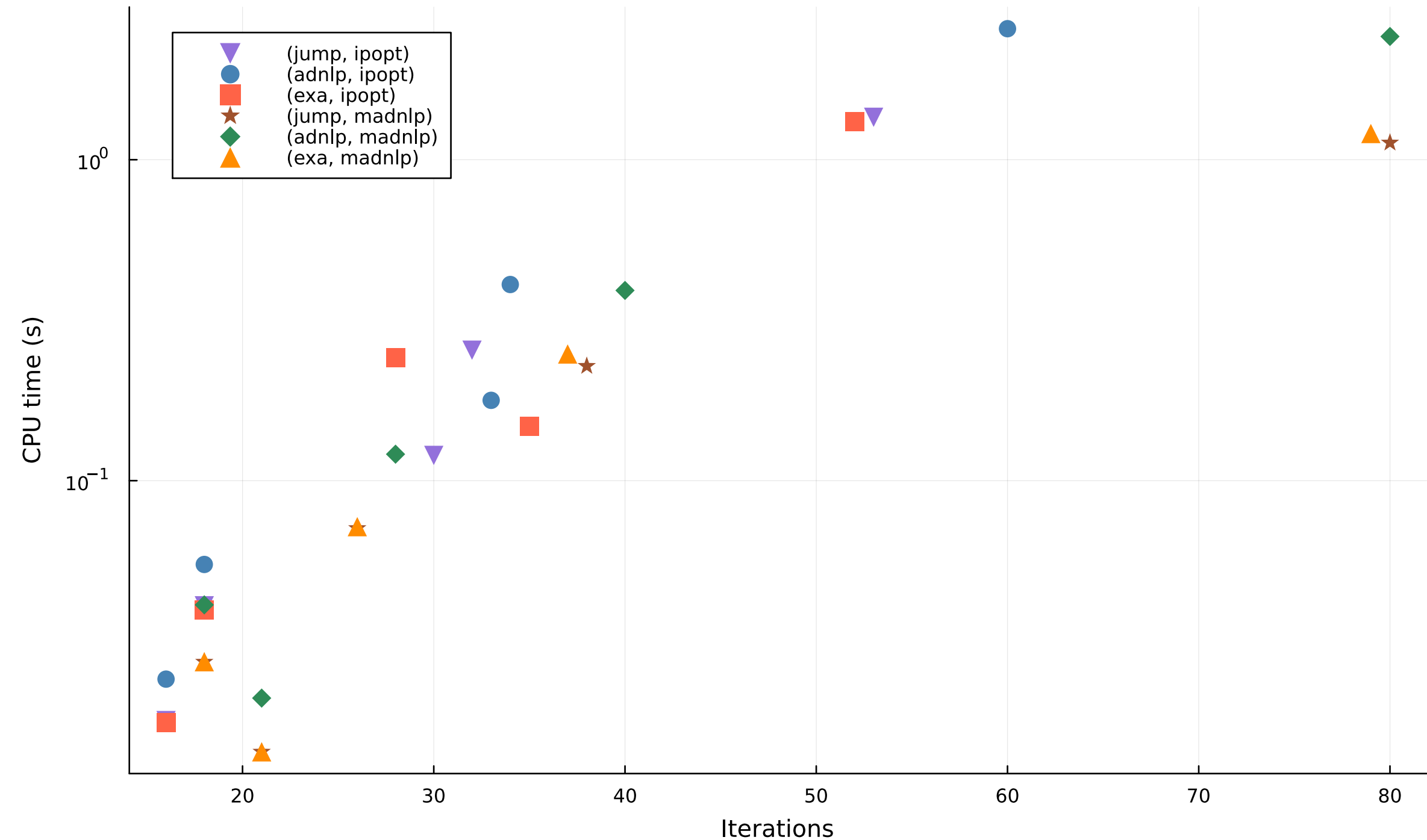
Iterations vs CPU time — beam
