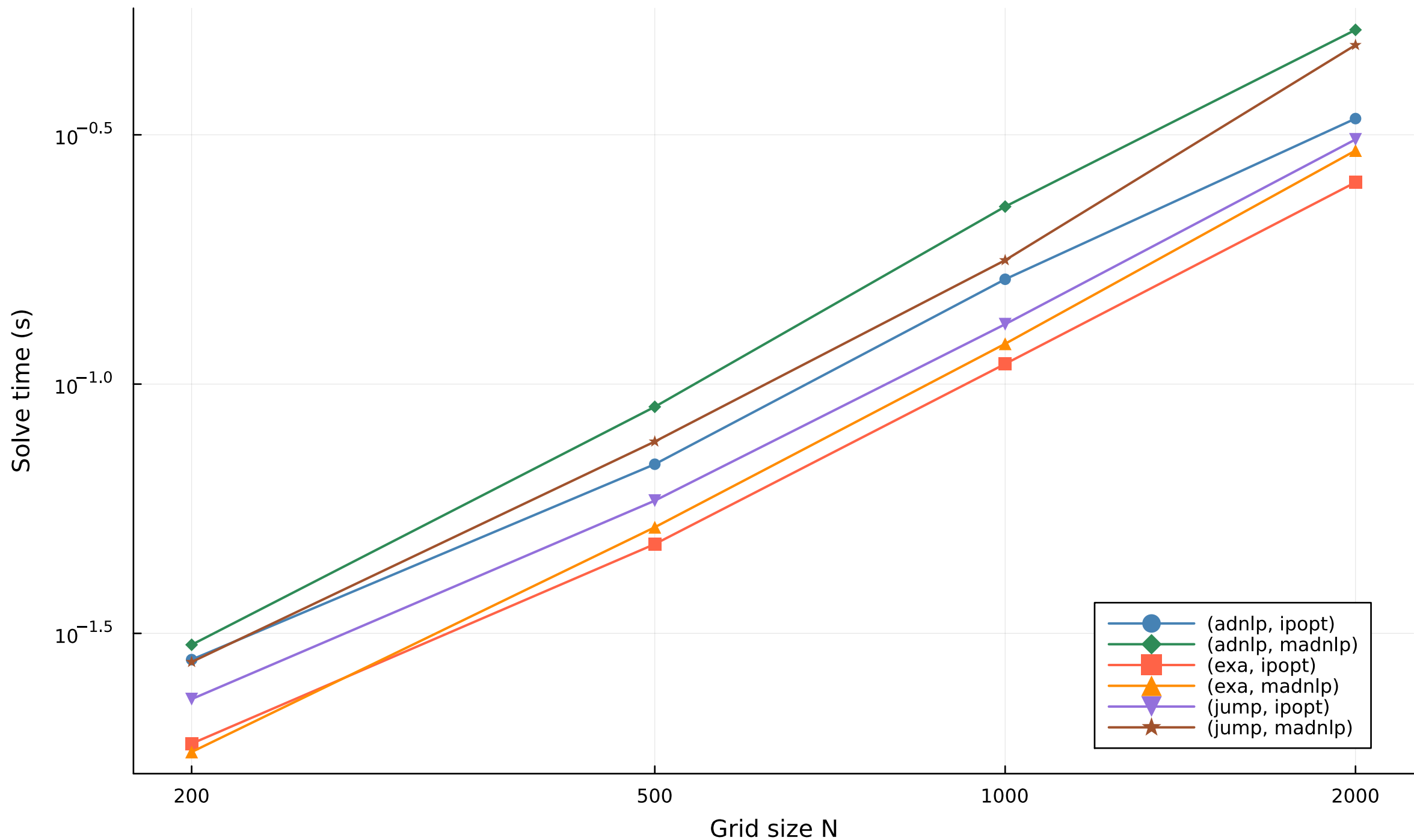
Solve time vs grid size — steering
