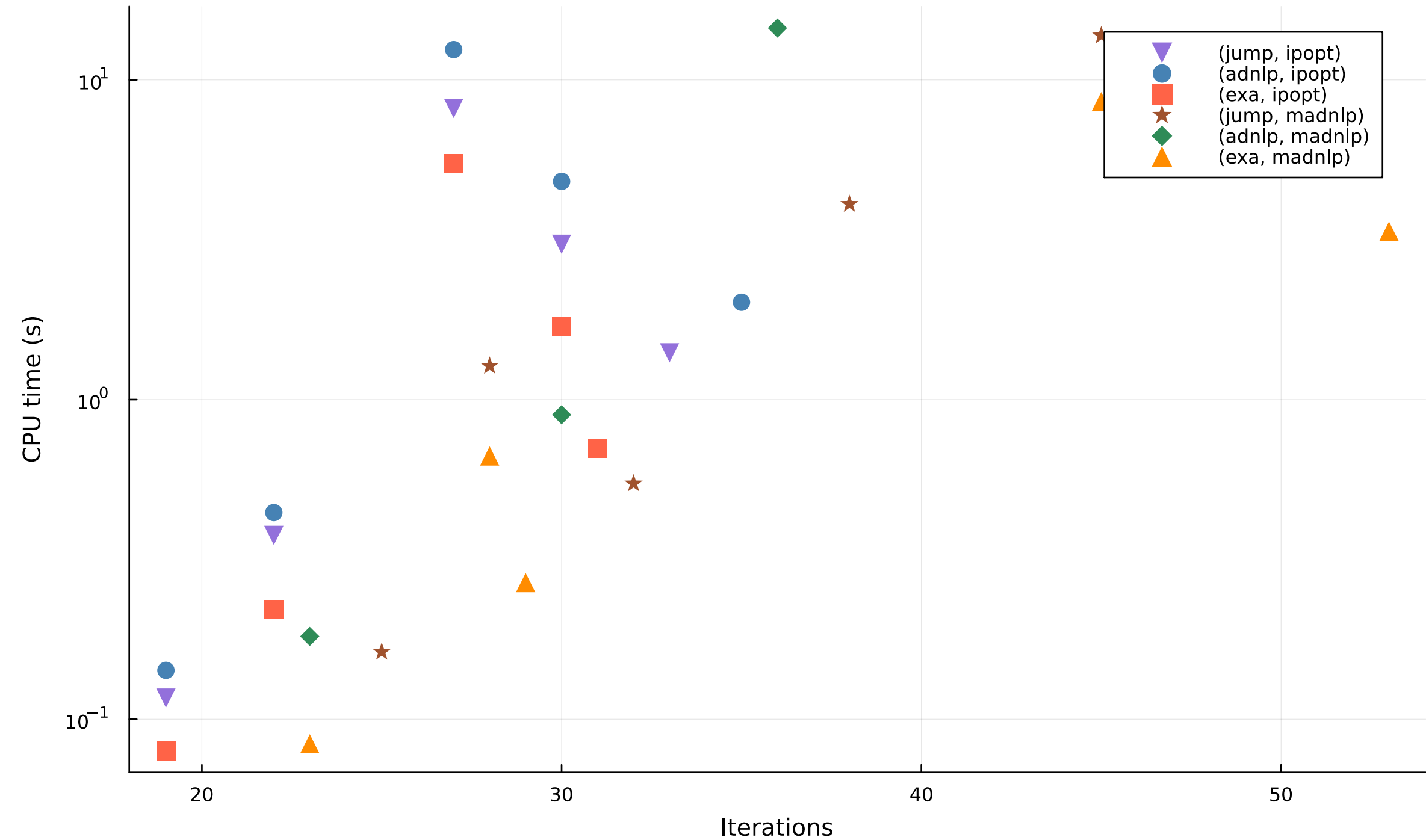
Iterations vs CPU time — robot
