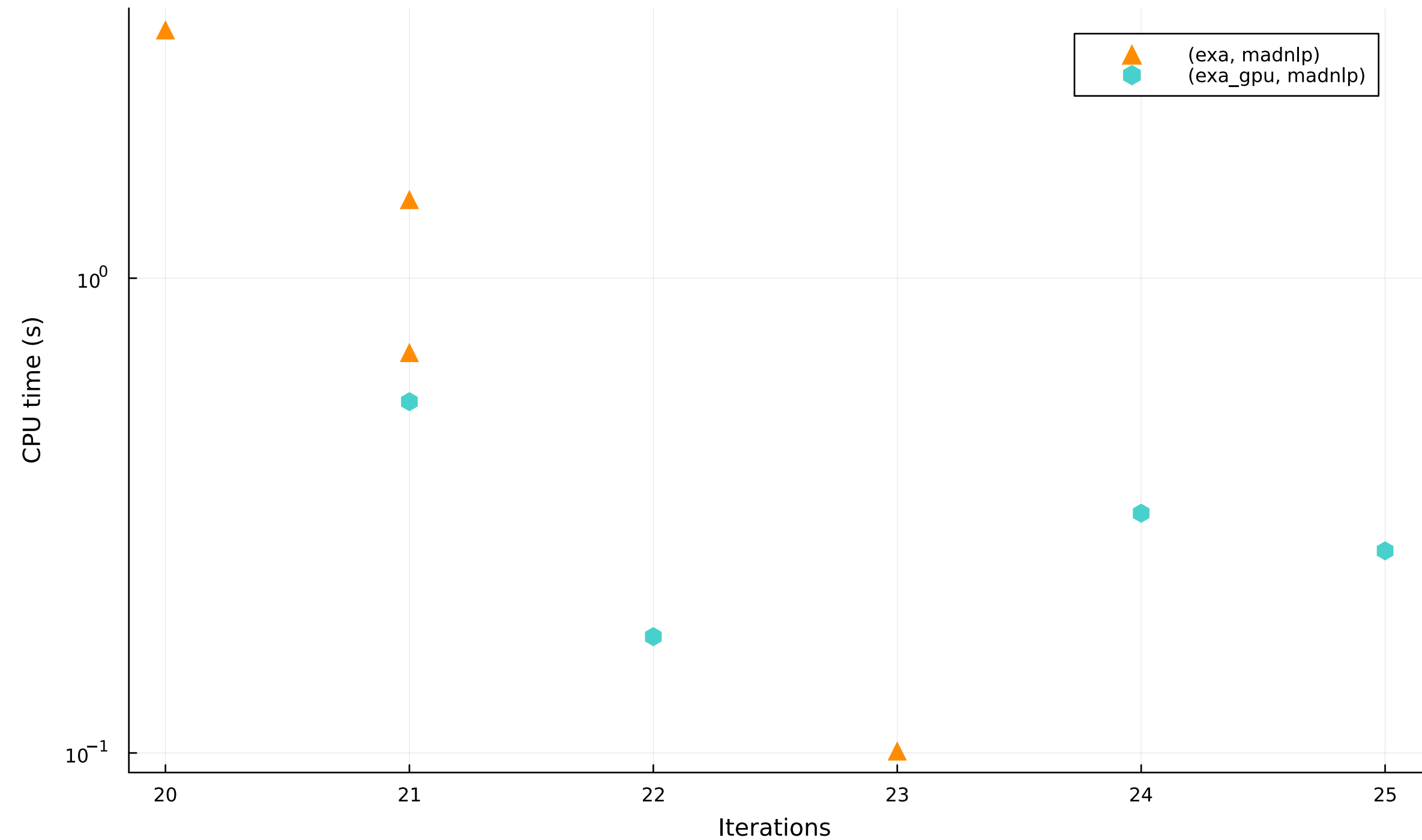
Iterations vs CPU time — jackson
