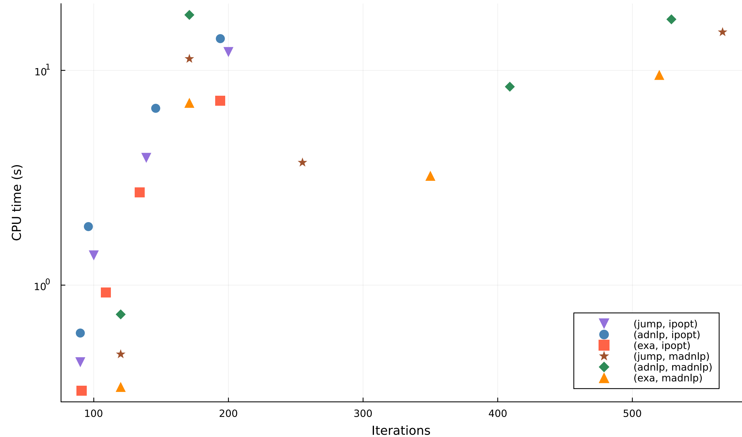
Iterations vs CPU time — insurance
