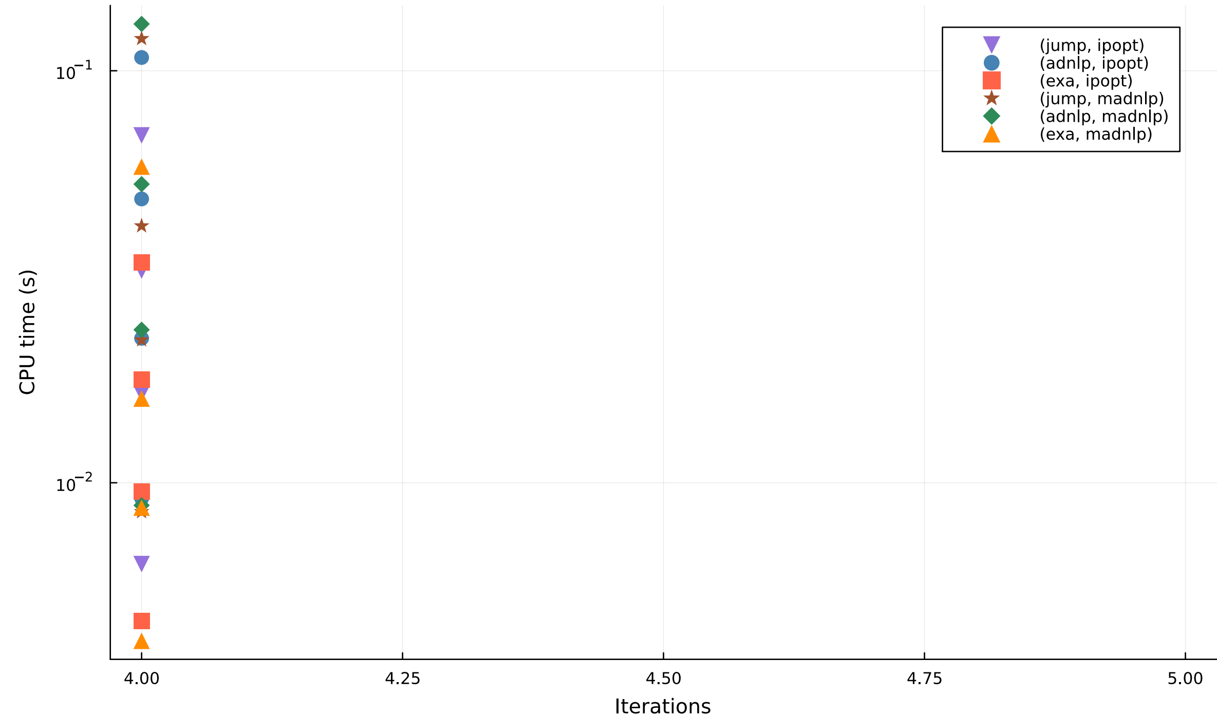
Iterations vs CPU time — electric_vehicle
