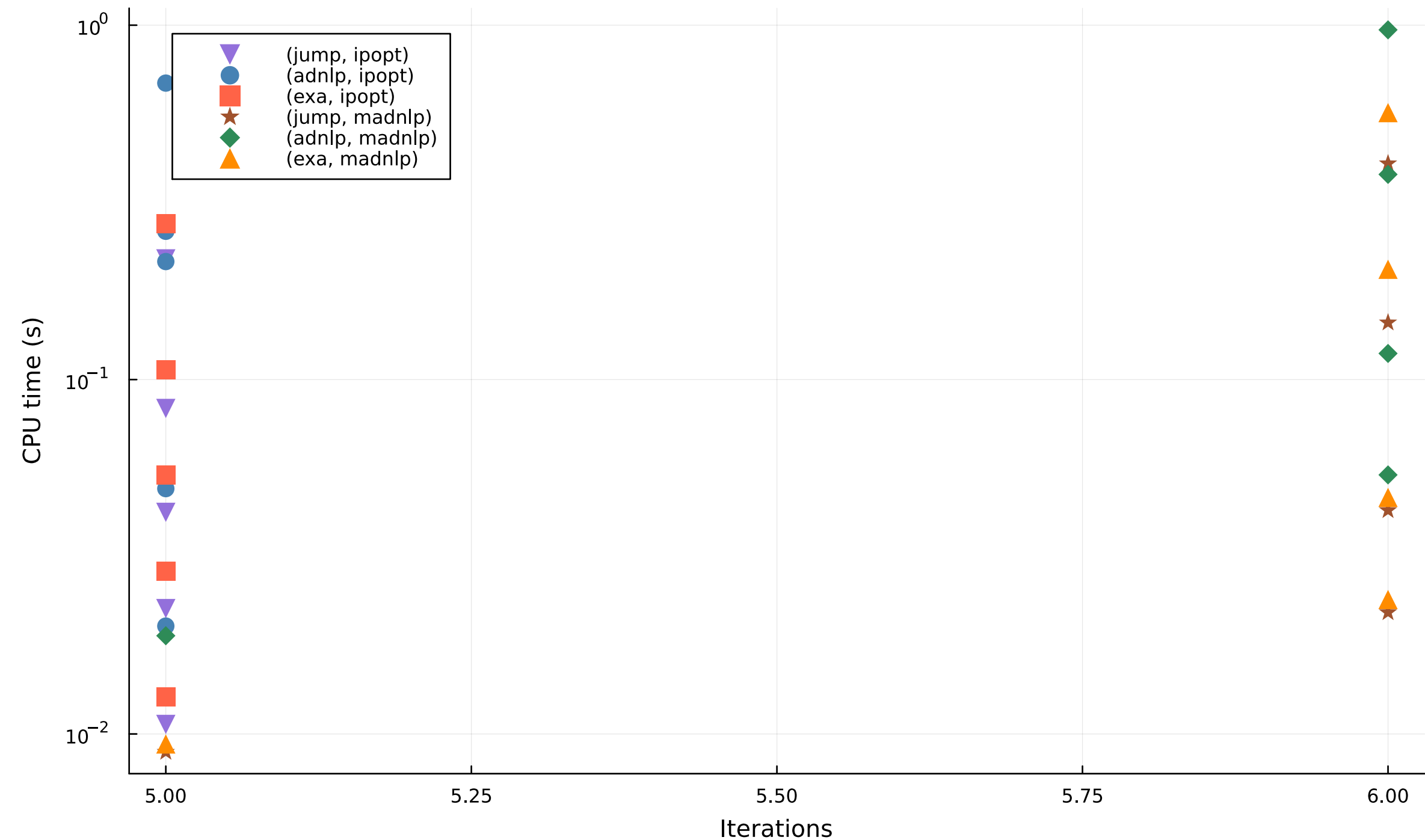
Iterations vs CPU time — double_oscillator
