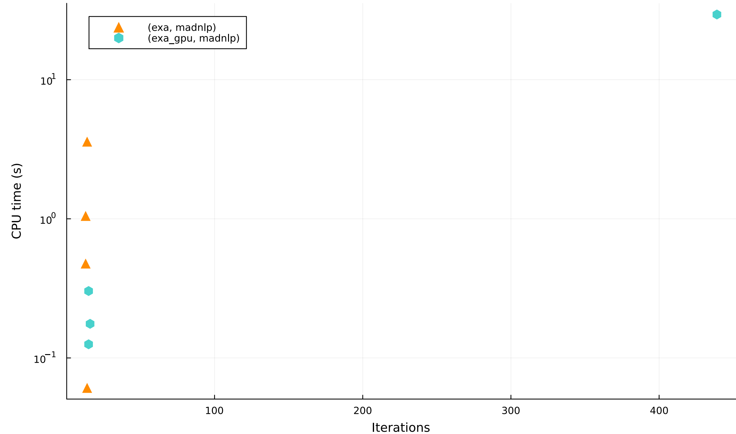
Iterations vs CPU time — chain
