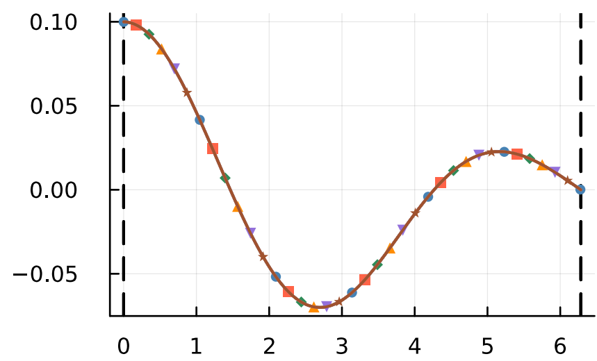
costate
