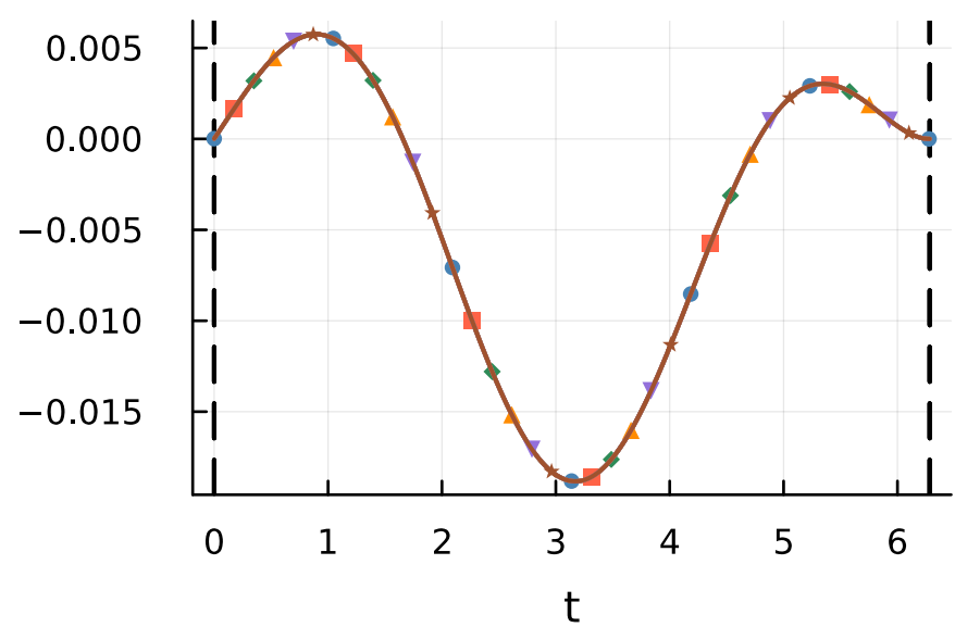
control
