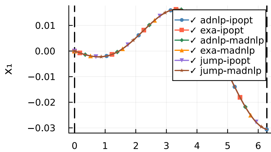
state
