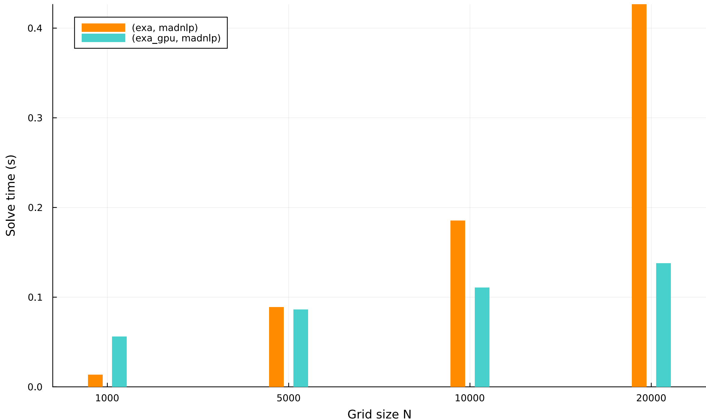
Solve time vs grid size (bar) — vanderpol
