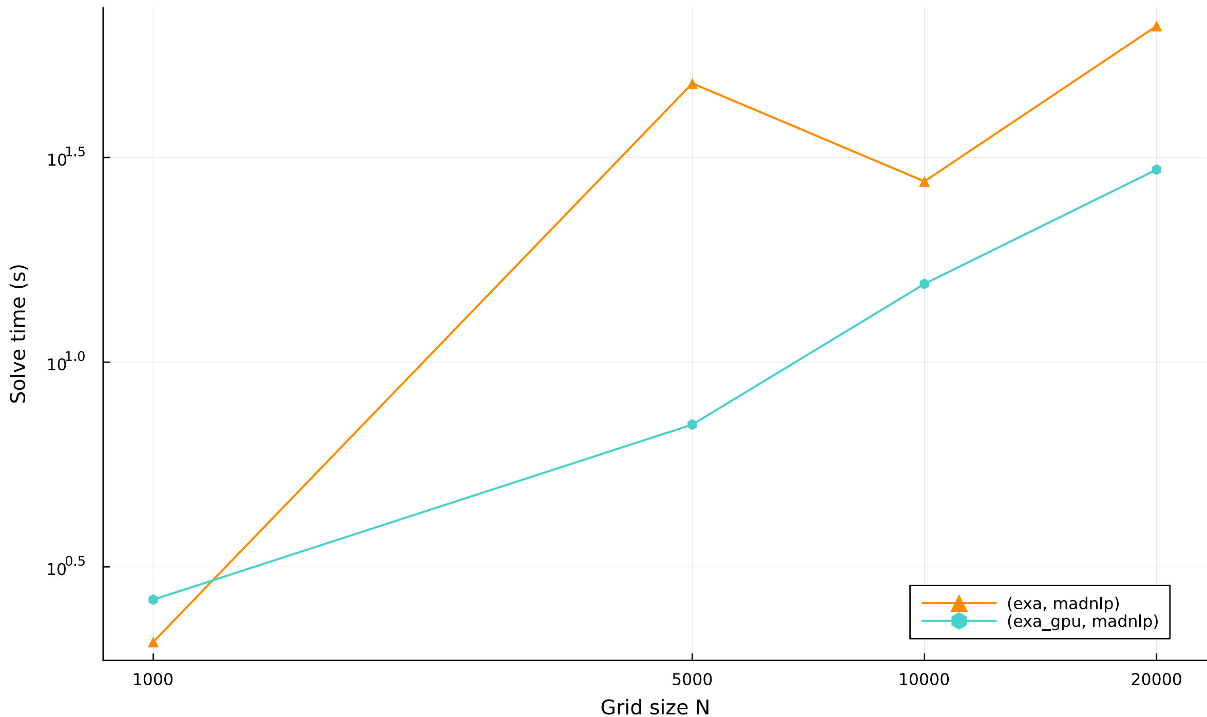
Solve time vs grid size — space_shuttle
