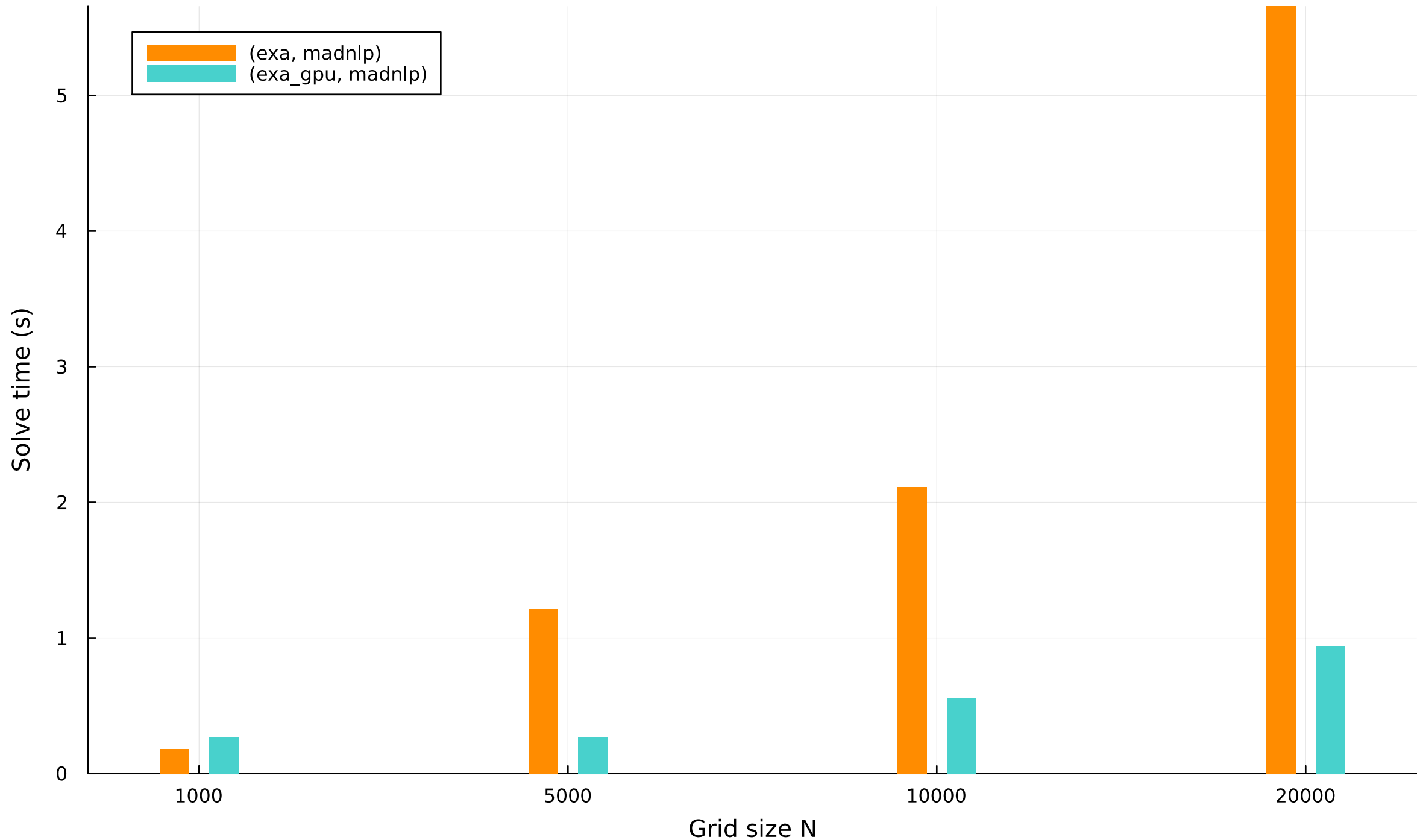
Solve time vs grid size (bar) — robbins
