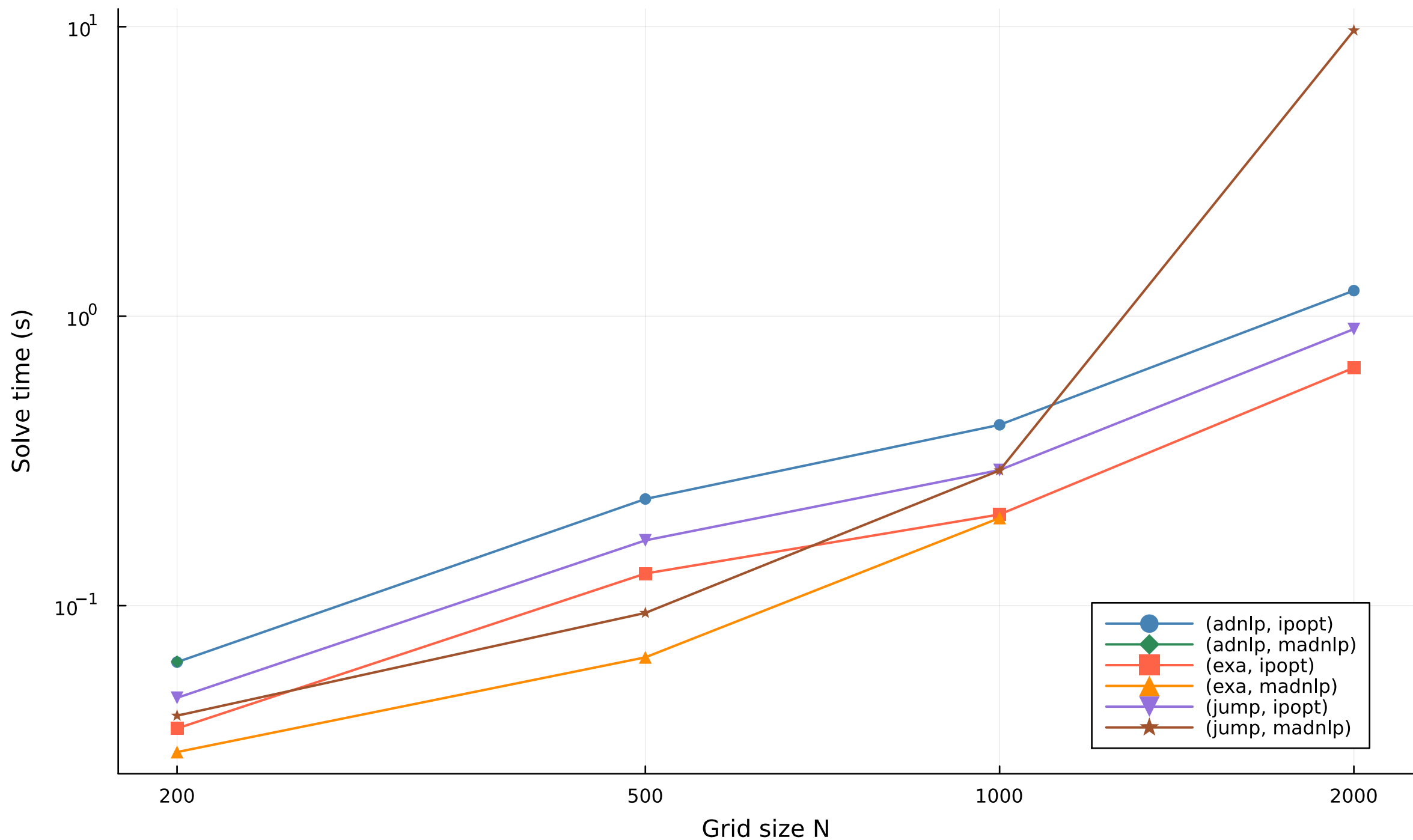
Solve time vs grid size — mountain_car
