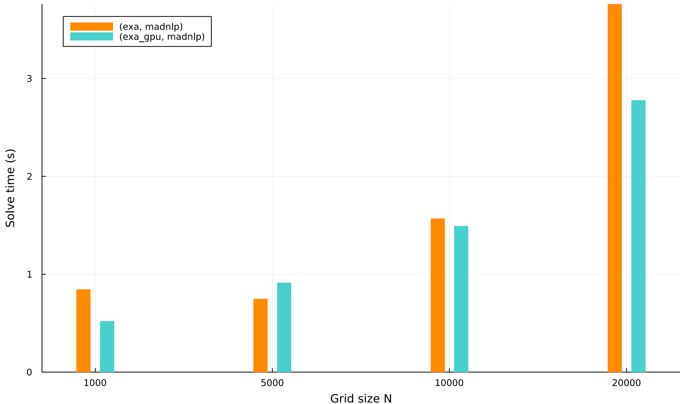
Solve time vs grid size (bar) — glider
