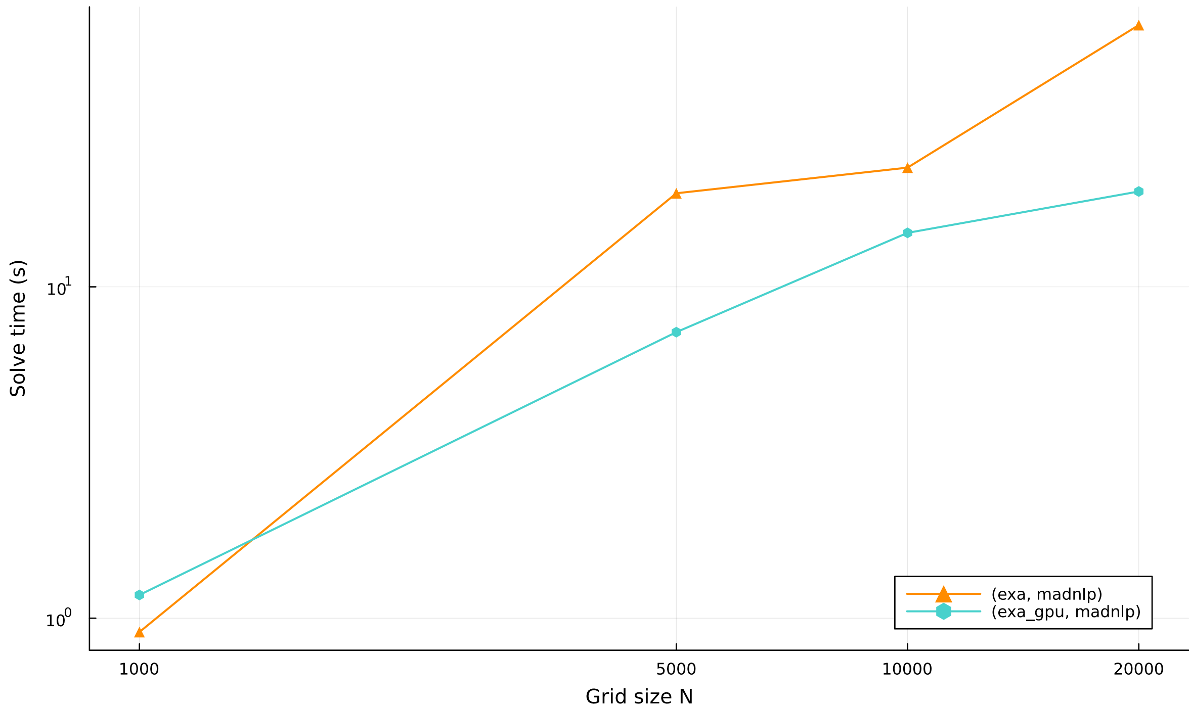
Solve time vs grid size — ducted_fan
