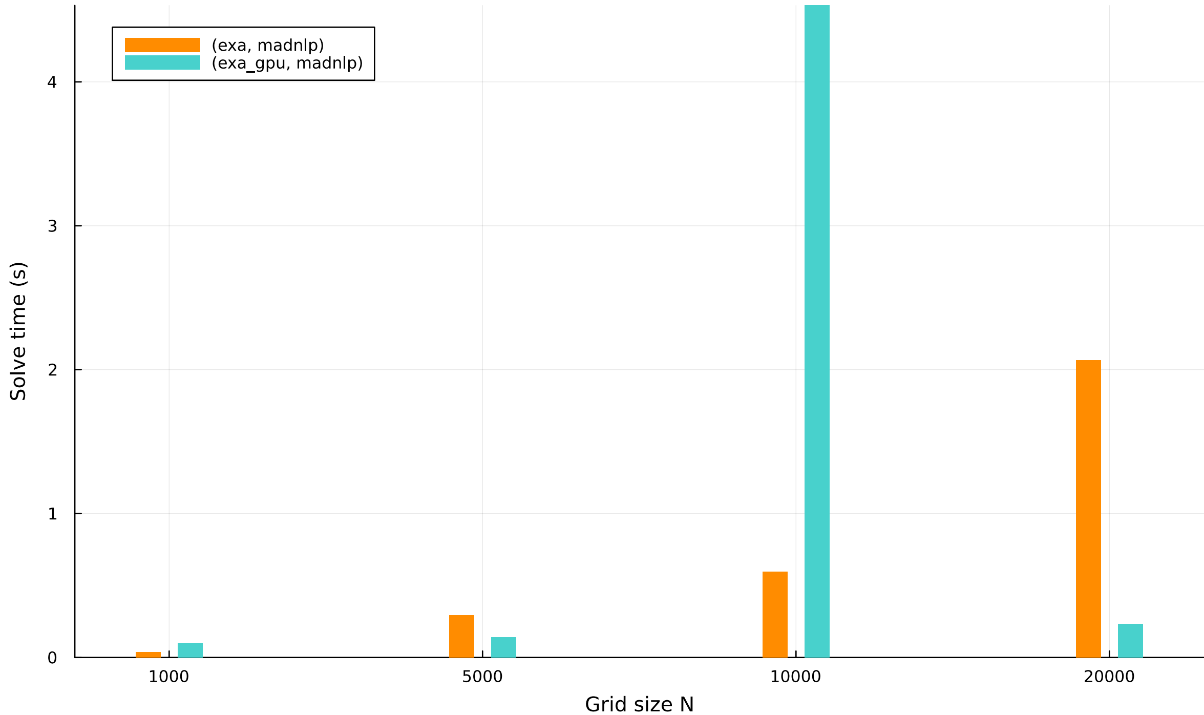
Solve time vs grid size (bar) — chain
