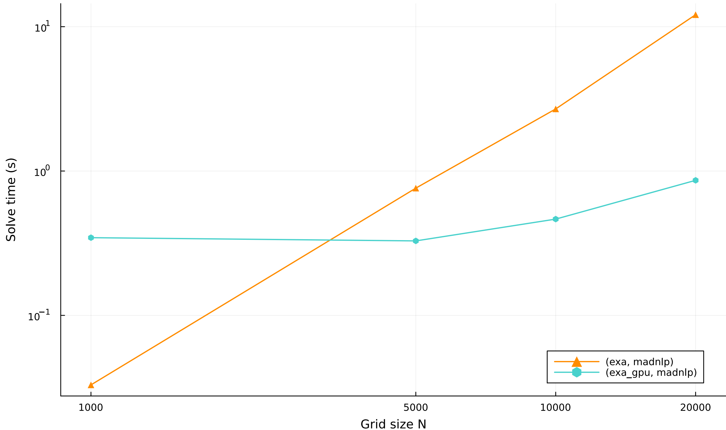
Solve time vs grid size — bryson_denham
