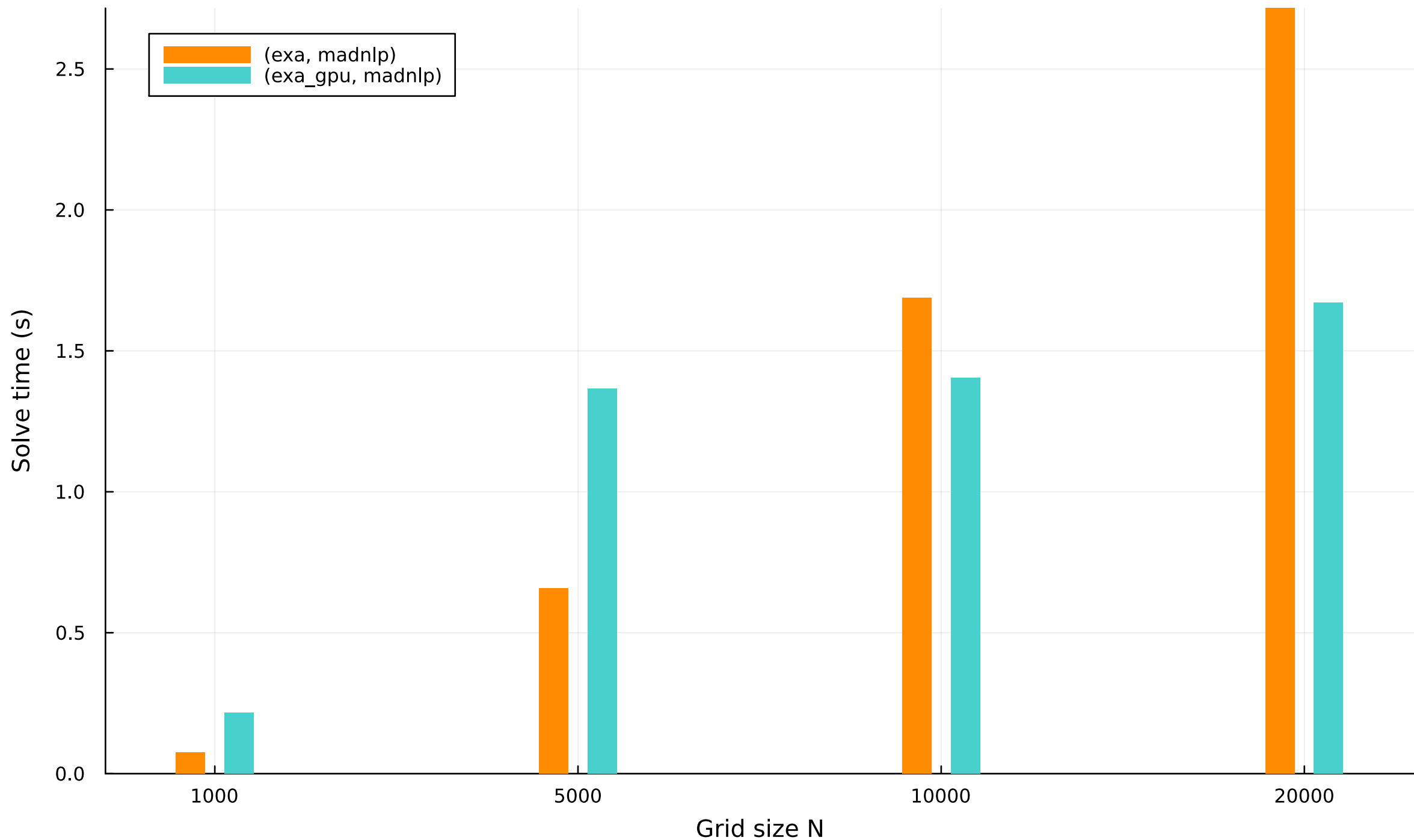
Solve time vs grid size (bar) — brachistochrone
