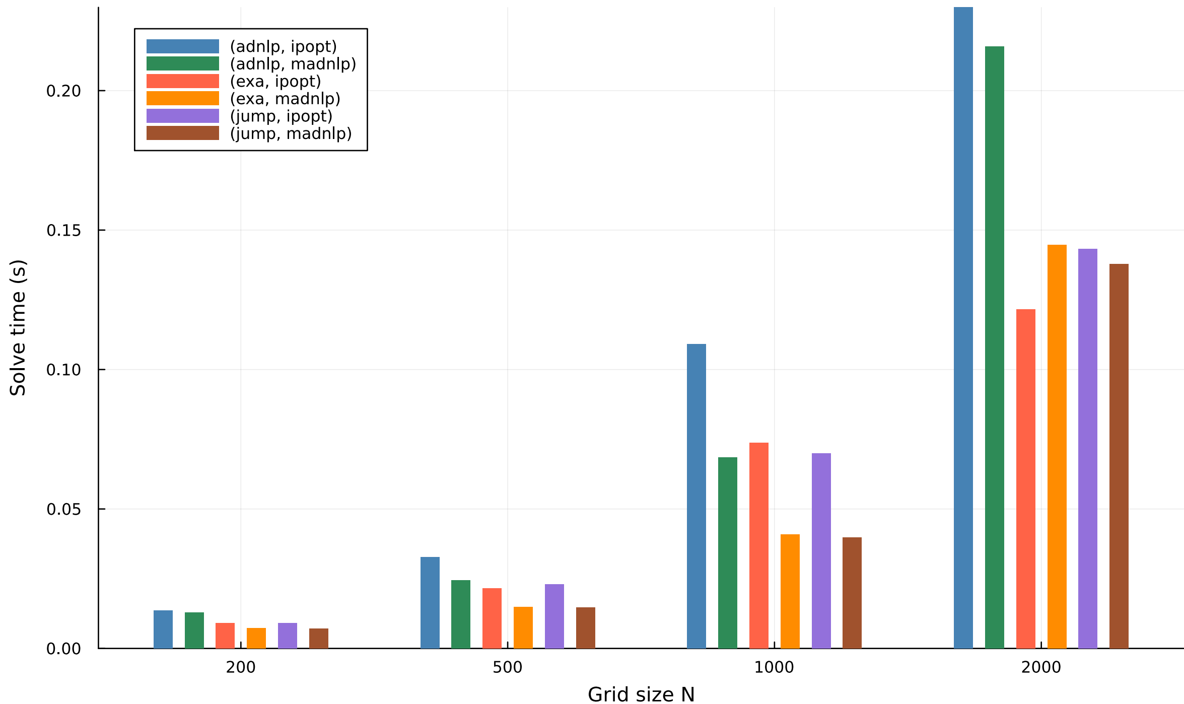
Solve time vs grid size (bar) — beam
